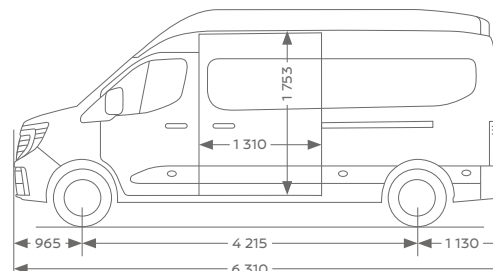
FOURGON L3 H2 & L3 H3
