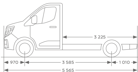
PLANCHER L2 H1
