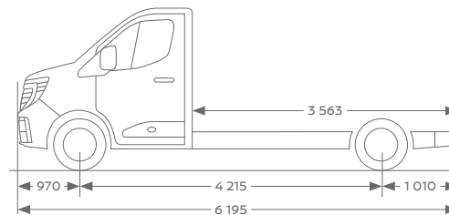
PLANCHER L3 H1
